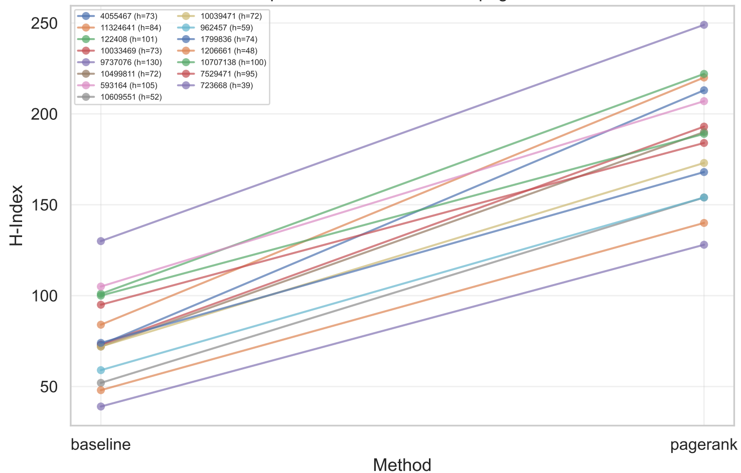
Top 15 Gainers - baseline -> pagerank
