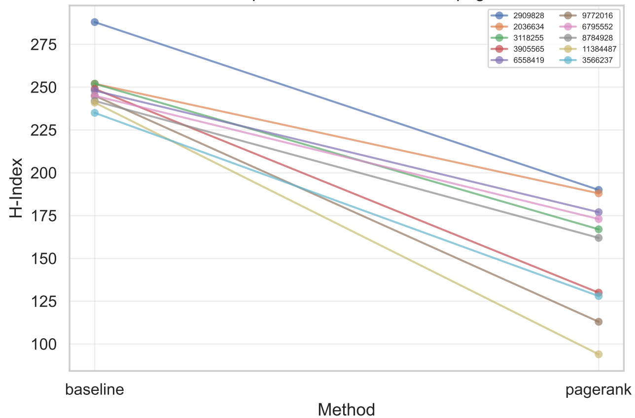
H-Index: Top-10 Authors - baseline -> pagerank
