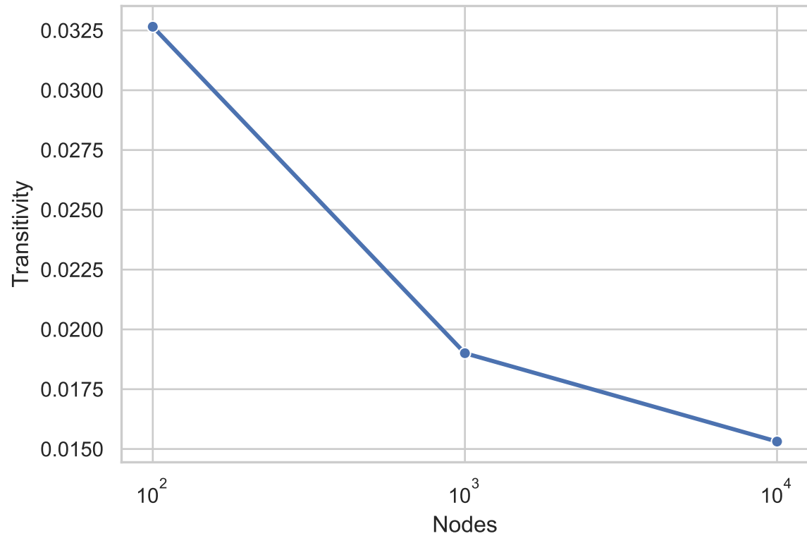
Transitivity vs Graph Size
