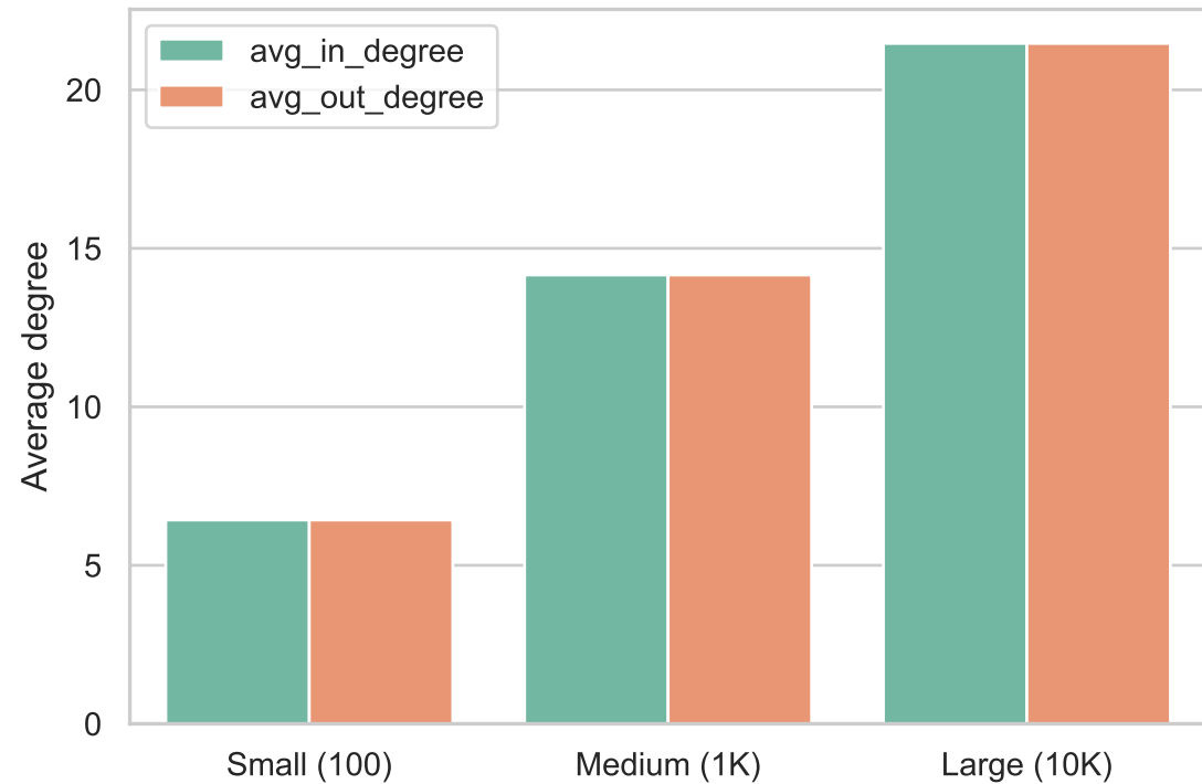
Average Degree by Graph Size
