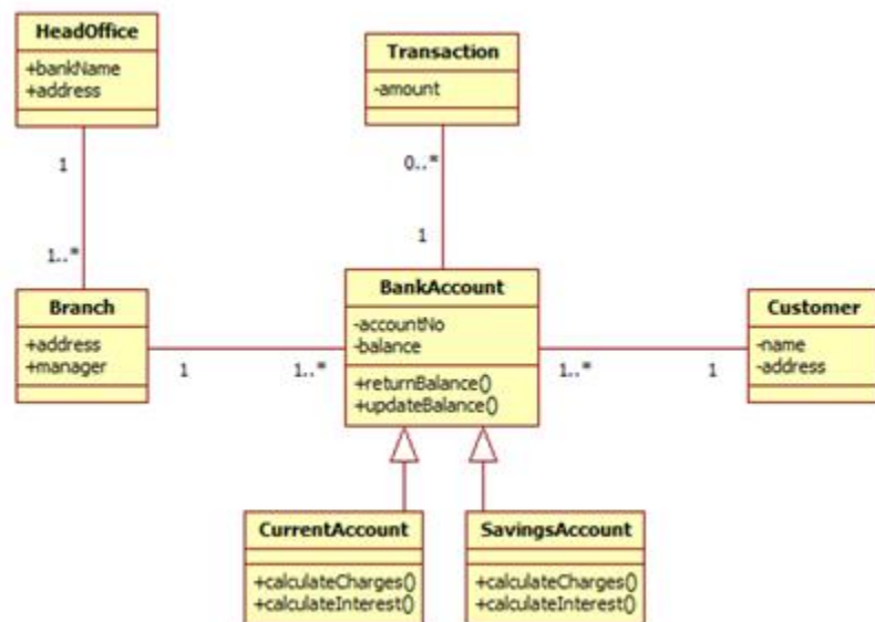
Banking Class Diagram
