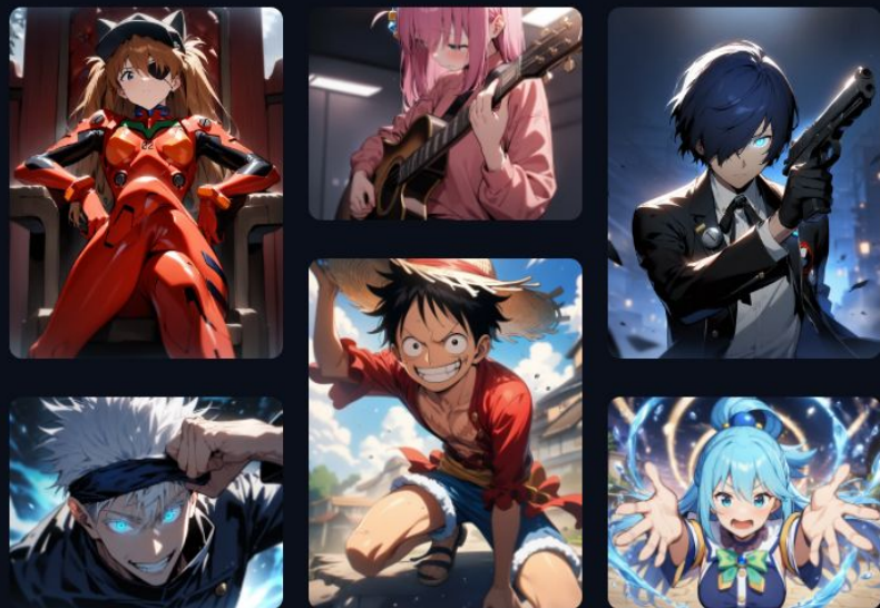
Anime model
