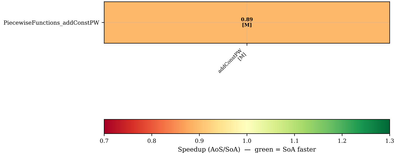
PiecewiseFunctions_addConstPW: per-pass speedup heatmap (F=fold M=map ?=unknown | SoA=7 buffers total)
