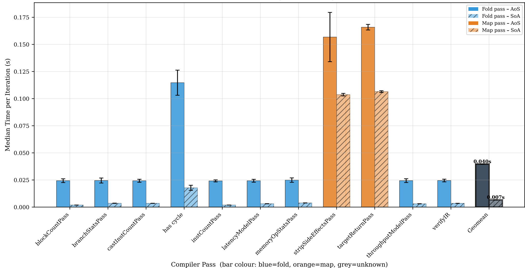
Compiler — AoS (solid) vs SoA (hatched), all passes (error bars = std dev, rightmost bar = geomean)
