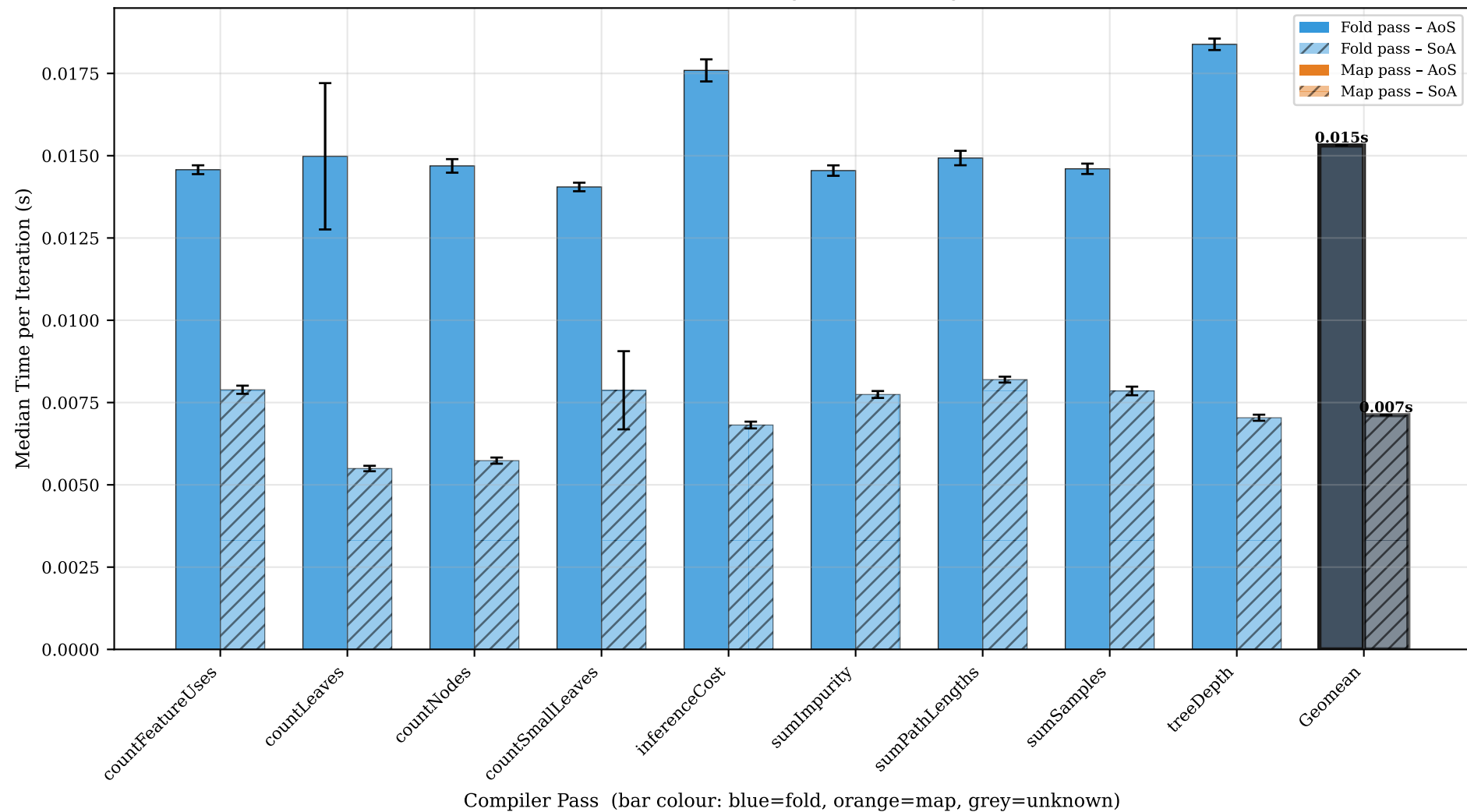
DecisionTree — AoS (solid) vs SoA (hatched), all passes (error bars = std dev, rightmost bar = geomean)
