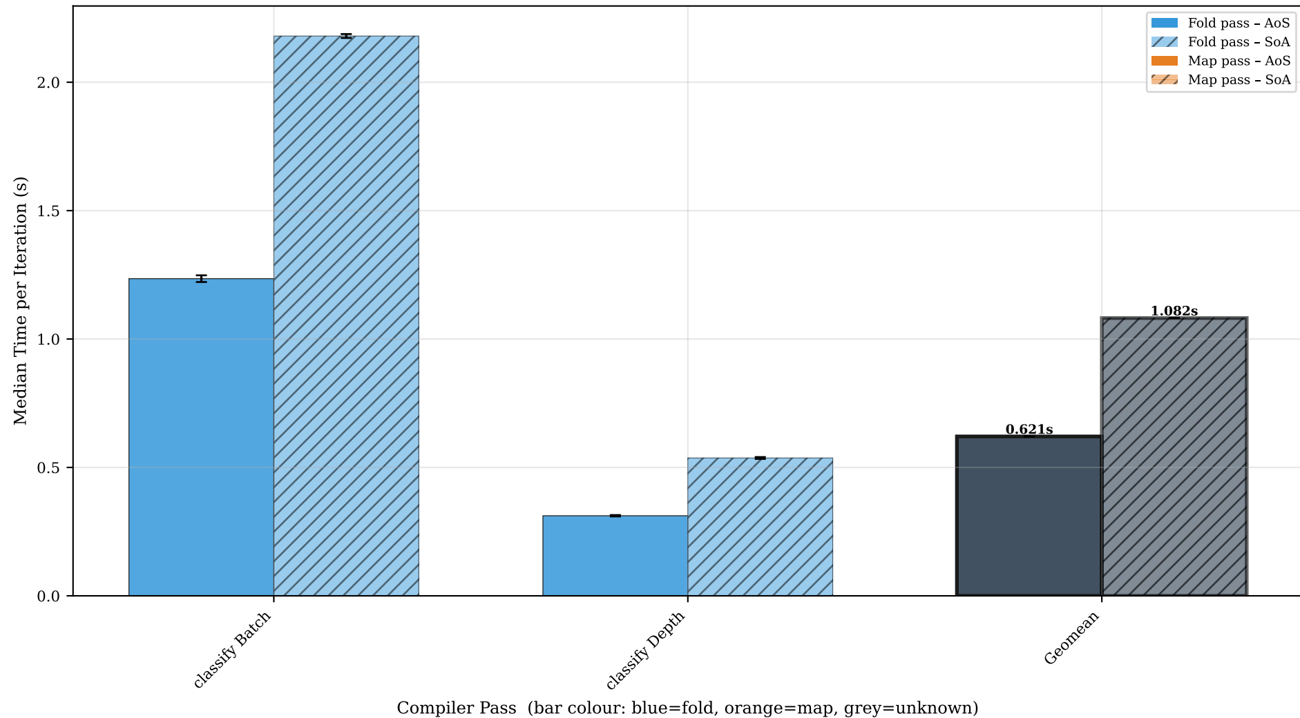
DecisionTreeClassify — AoS (solid) vs SoA (hatched), all passes (error bars = std dev, rightmost bar = geomean)
