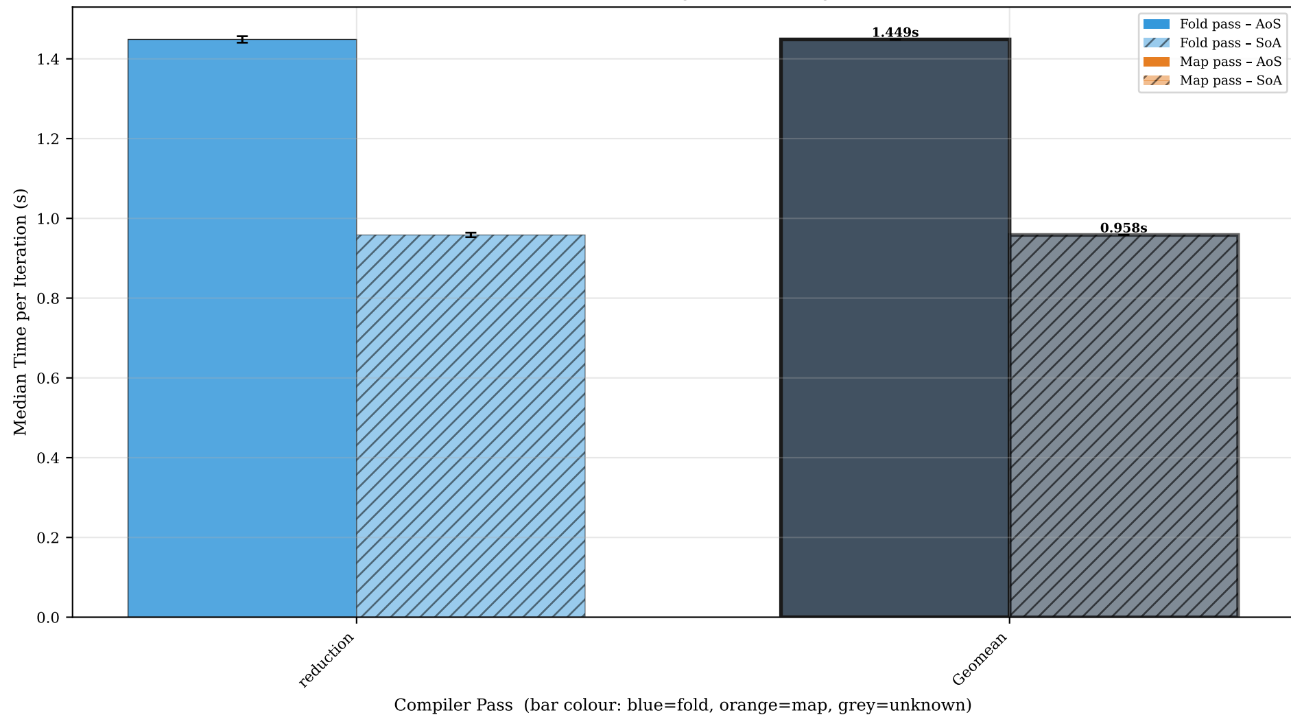
reduceNestedList — AoS (solid) vs SoA (hatched), all passes (error bars = std dev, rightmost bar = geomean)
