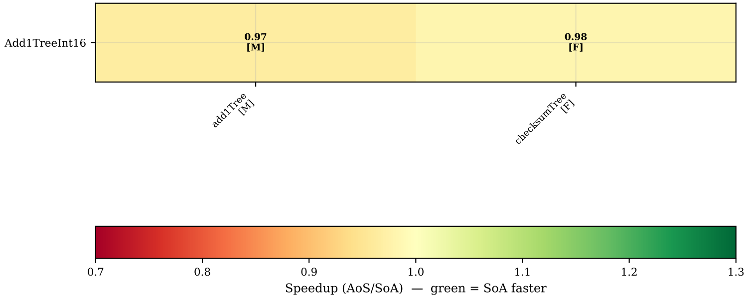
Add1TreeInt16: per-pass speedup heatmap (F=fold M=map ?=unknown | SoA=2 buffers total)
