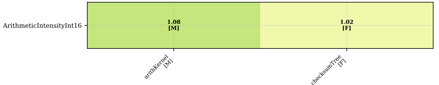
ArithmeticIntensityInt16: per-pass speedup heatmap (F=fold M=map ?=unknown | SoA=2 buffers total)
