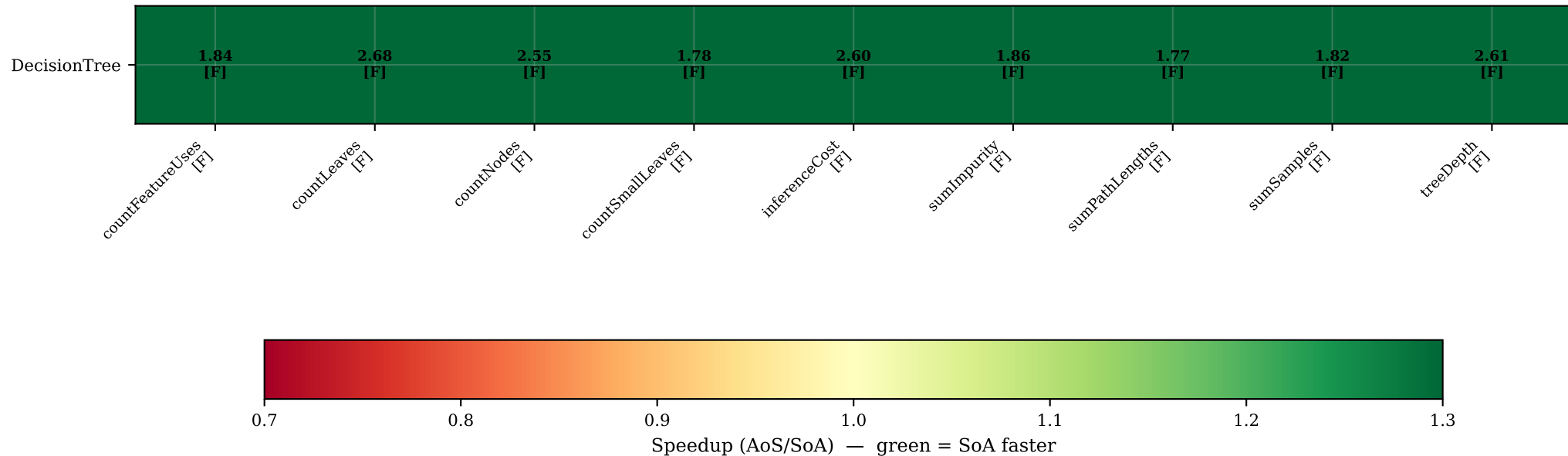
DecisionTree: per-pass speedup heatmap (F=fold M=map ?=unknown | SoA=6 buffers total)
