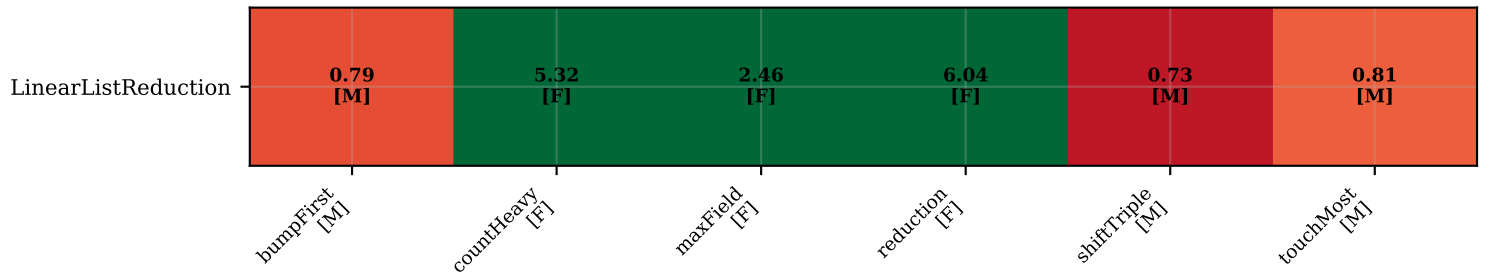
LinearListReduction: per-pass speedup heatmap (F=fold M=map ?=unknown | SoA=11 buffers total)
