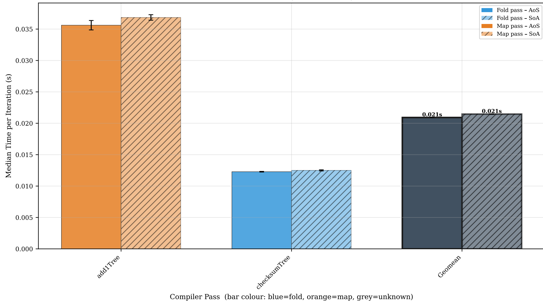
Add1TreeInt16 — AoS (solid) vs SoA (hatched), all passes (error bars = std dev, rightmost bar = geomean)
