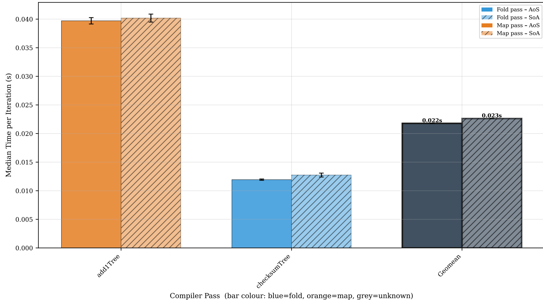
Add1TreeInt32 — AoS (solid) vs SoA (hatched), all passes (error bars = std dev, rightmost bar = geomean)
