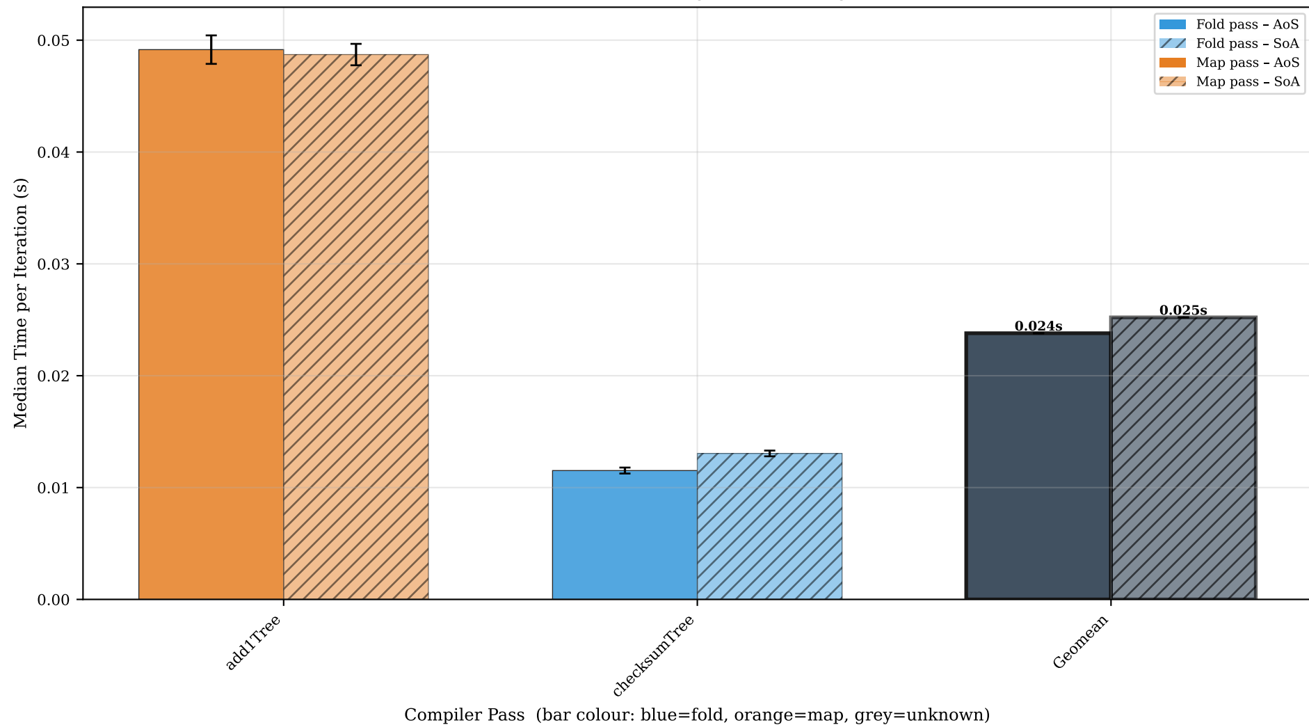
Add1TreeInt64 — AoS (solid) vs SoA (hatched), all passes (error bars = std dev, rightmost bar = geomean)
