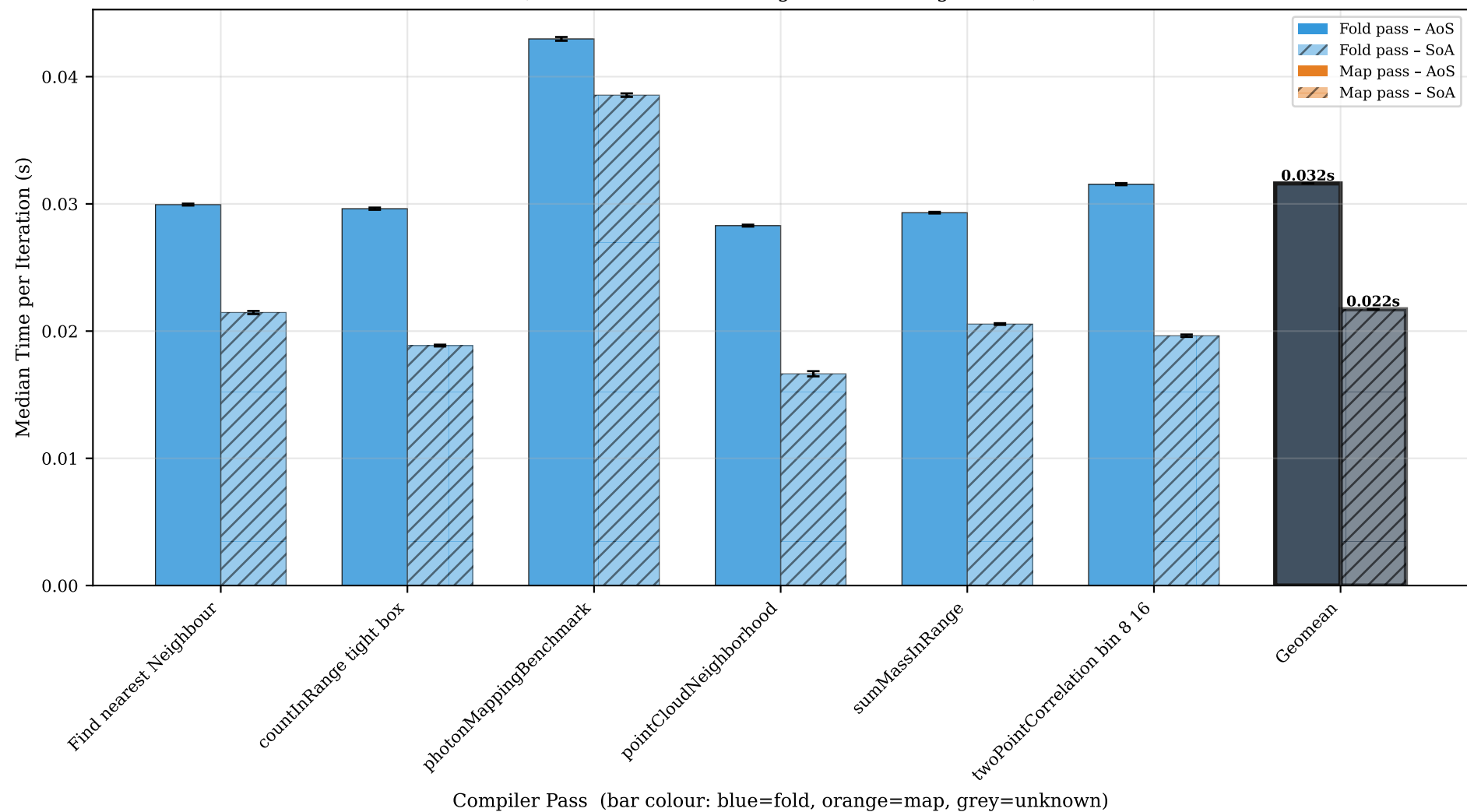
KDTree — AoS (solid) vs SoA (hatched), all passes (error bars = std dev, rightmost bar = geomean)
