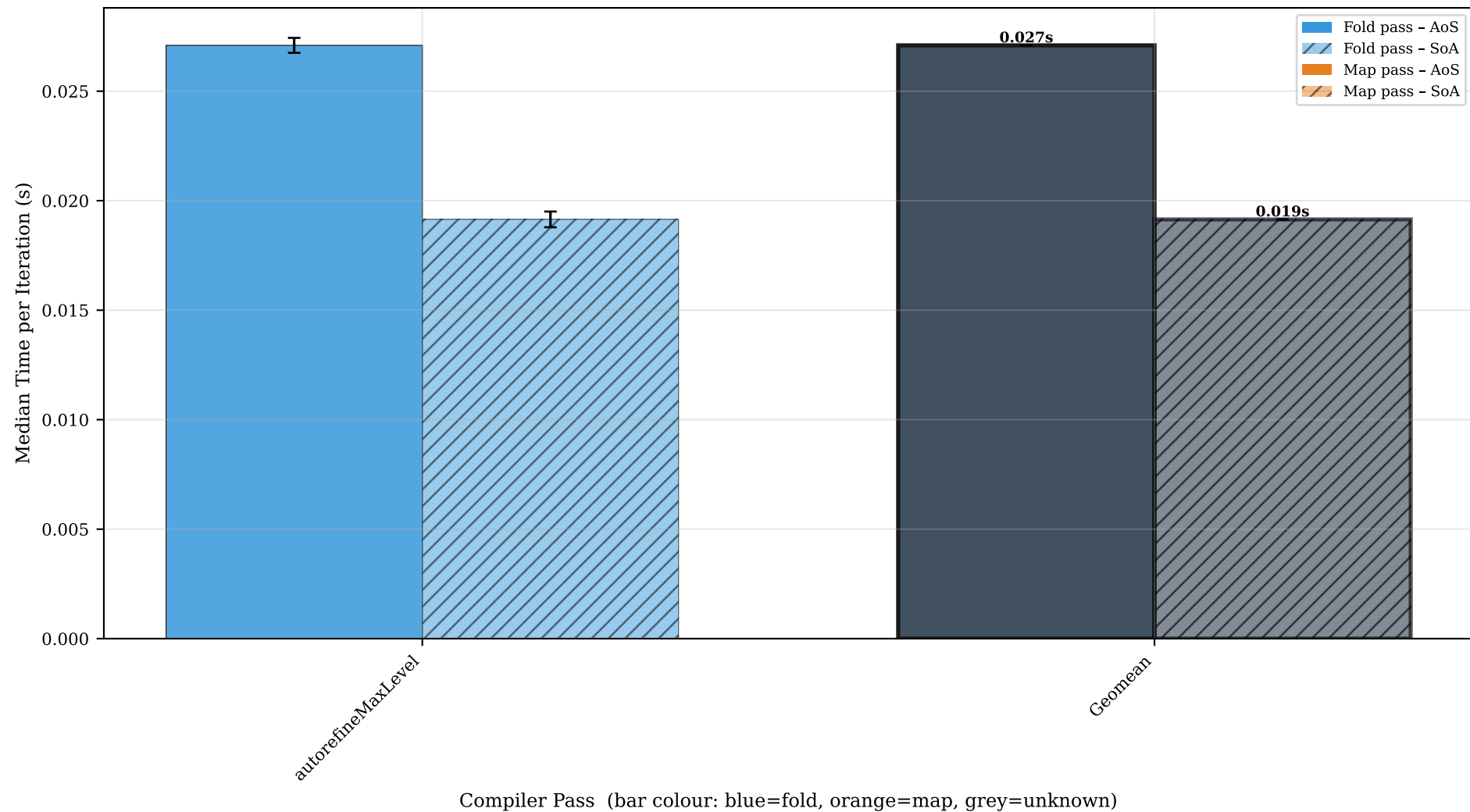
PiecewiseFunctions_autorefineMaxLevel — AoS (solid) vs SoA (hatched), all passes (error bars = std dev, rightmost bar = geomean)
