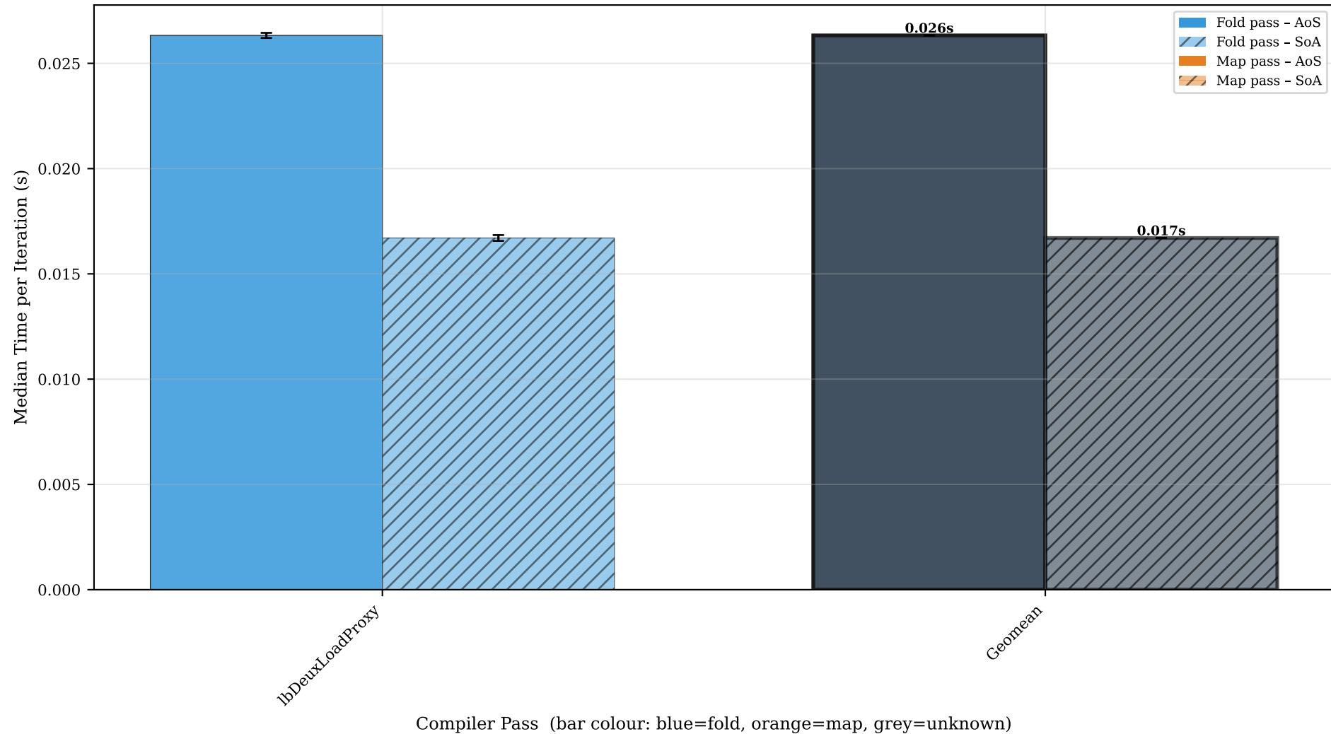
PiecewiseFunctions_lbDeuxLoadProxy — AoS (solid) vs SoA (hatched), all passes (error bars = std dev, rightmost bar = geomean)
