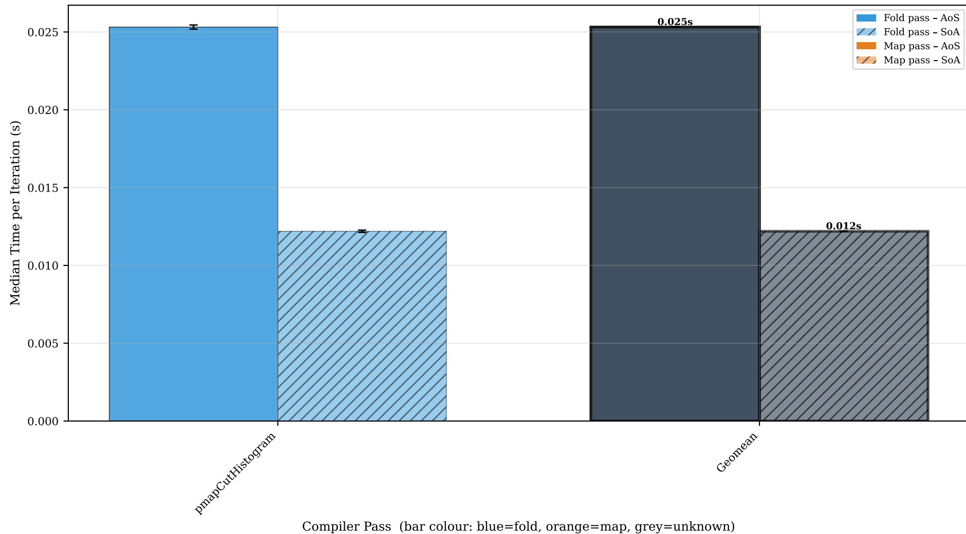
PiecewiseFunctions_pmapCutHistogram — AoS (solid) vs SoA (hatched), all passes (error bars = std dev, rightmost bar = geomean)
