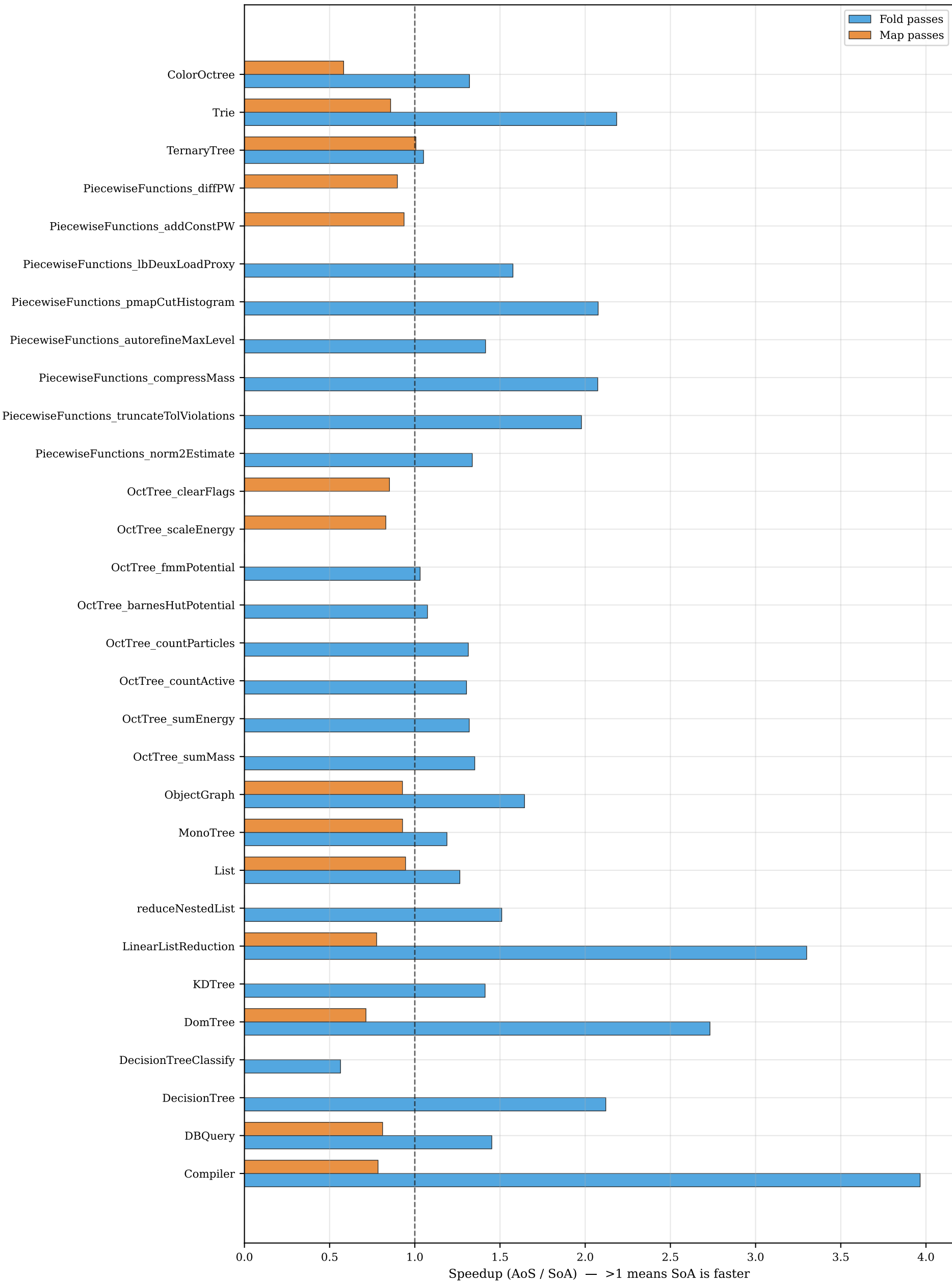
End-to-End Speedup: Fold vs Map Passes
