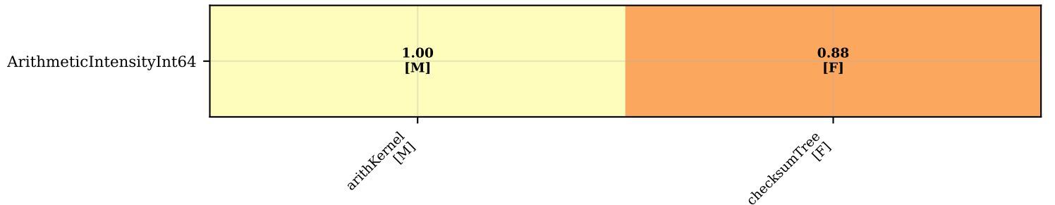
ArithmeticIntensityInt64: per-pass speedup heatmap (F=fold M=map ?=unknown | SoA=2 buffers total)
