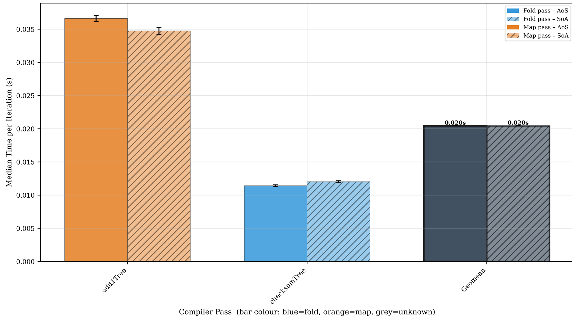
Add1TreeInt8 — AoS (solid) vs SoA (hatched), all passes (error bars = std dev, rightmost bar = geomean)
