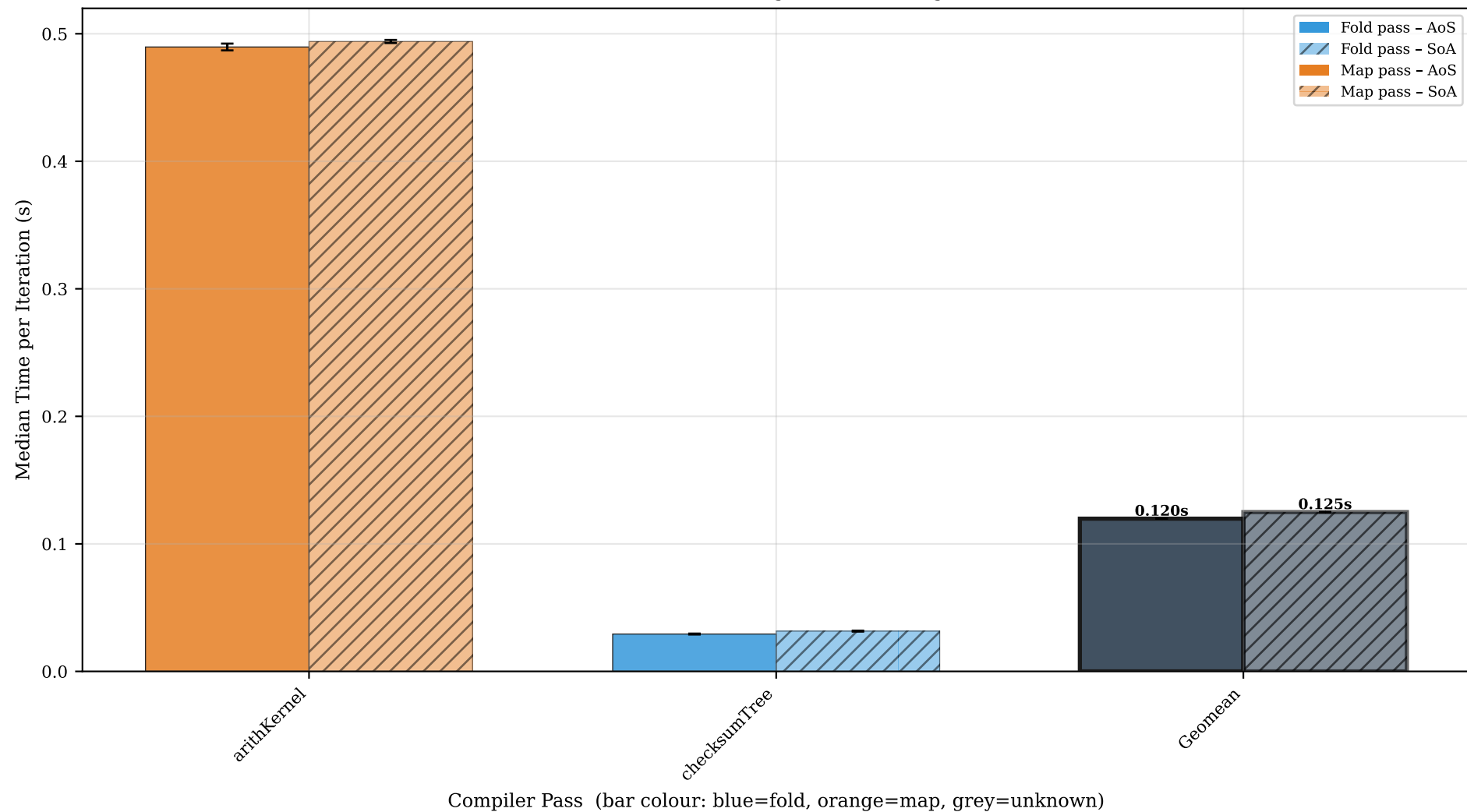
ArithmeticIntensityInt16 — AoS (solid) vs SoA (hatched), all passes (error bars = std dev, rightmost bar = geomean)
