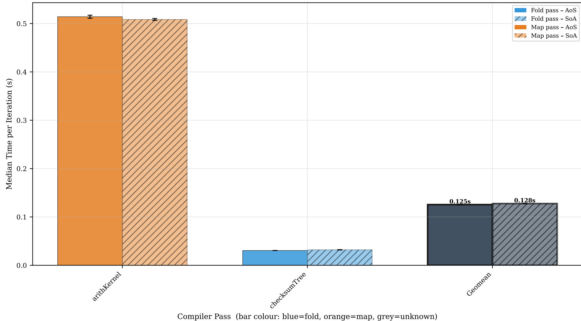
ArithmeticIntensityInt32 — AoS (solid) vs SoA (hatched), all passes (error bars = std dev, rightmost bar = geomean)
