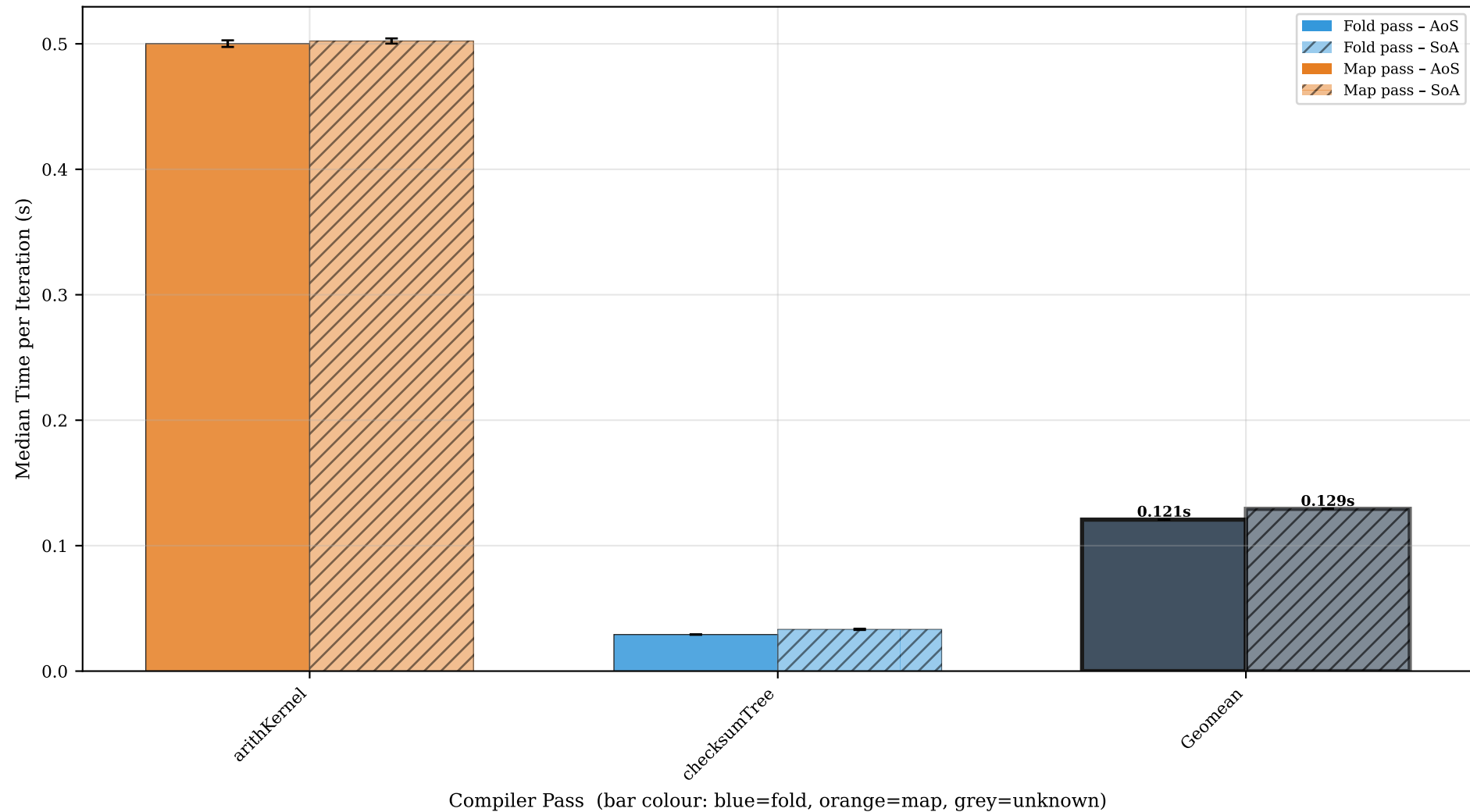
ArithmeticIntensityInt64 — AoS (solid) vs SoA (hatched), all passes (error bars = std dev, rightmost bar = geomean)
