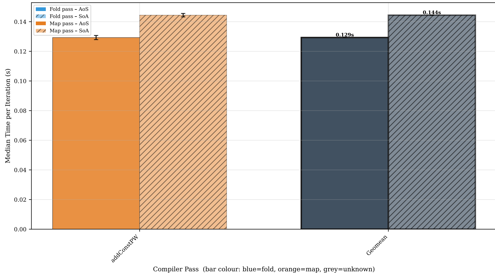
PiecewiseFunctions_addConstPW — AoS (solid) vs SoA (hatched), all passes (error bars = std dev, rightmost bar = geomean)
