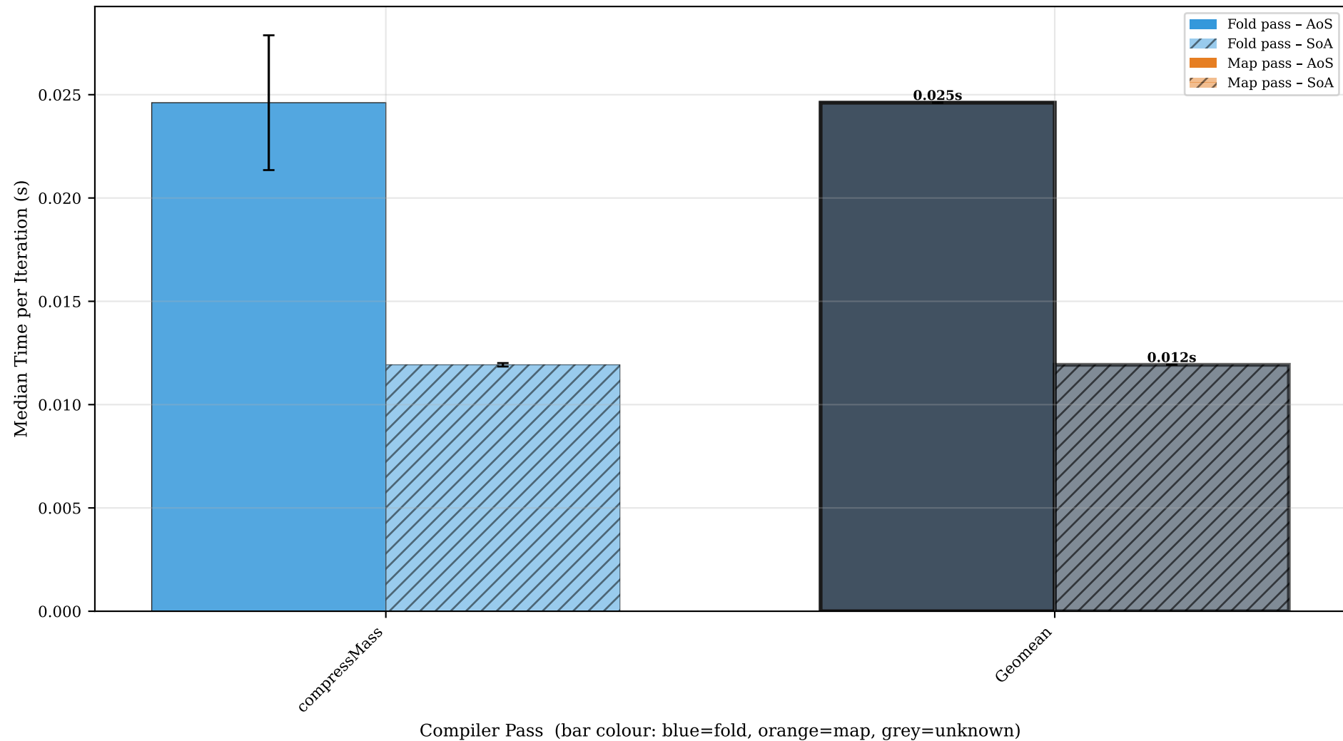
PiecewiseFunctions_compressMass — AoS (solid) vs SoA (hatched), all passes (error bars = std dev, rightmost bar = geomean)
