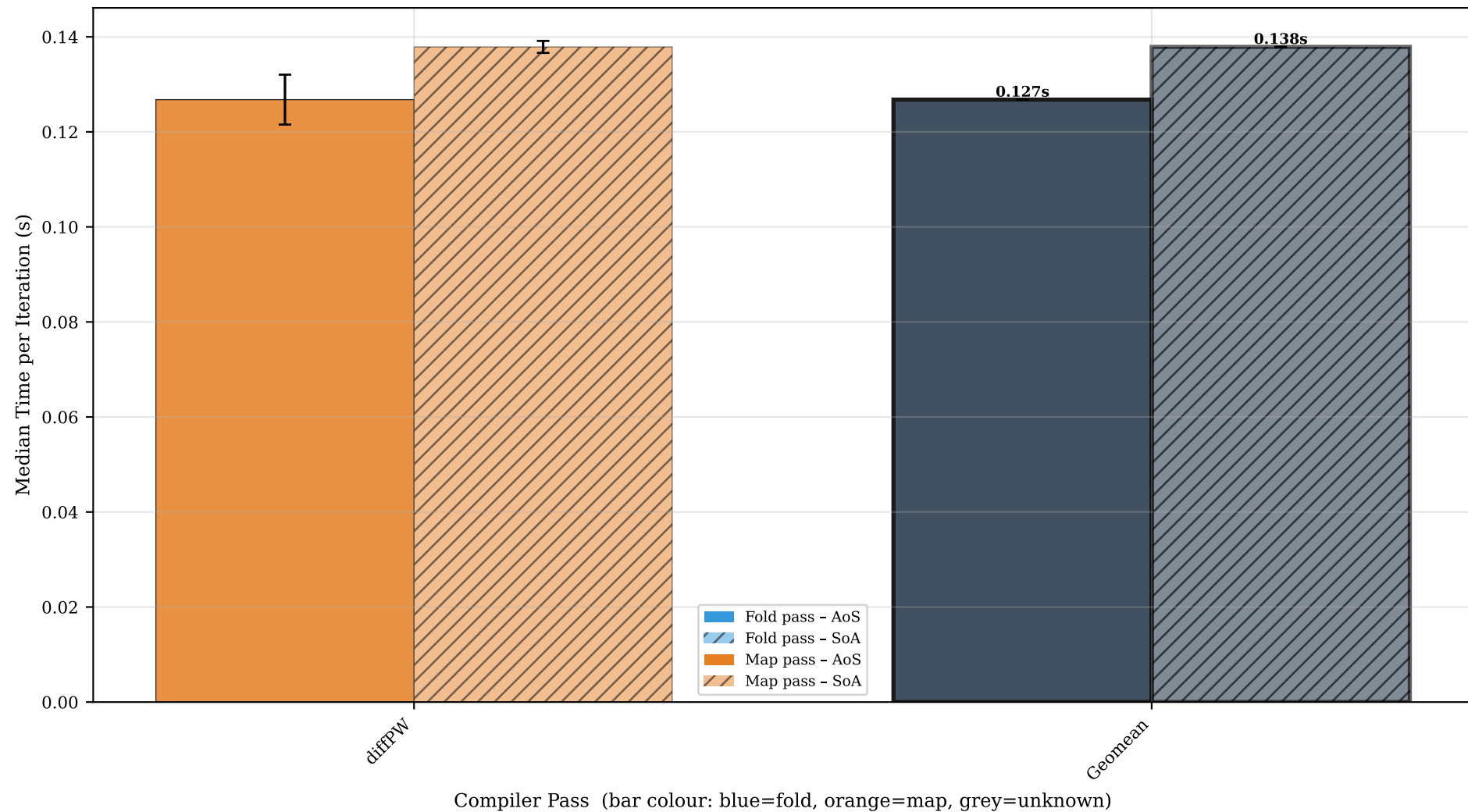
PiecewiseFunctions_diffPW — AoS (solid) vs SoA (hatched), all passes (error bars = std dev, rightmost bar = geomean)
