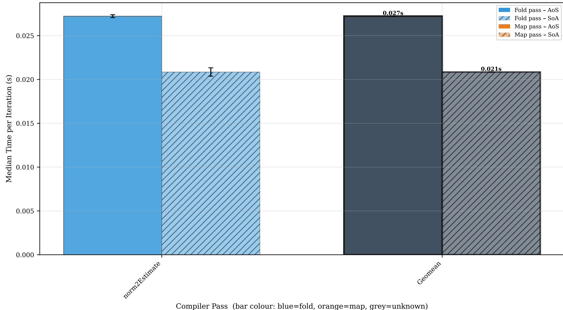
PiecewiseFunctions_norm2Estimate — AoS (solid) vs SoA (hatched), all passes (error bars = std dev, rightmost bar = geomean)
