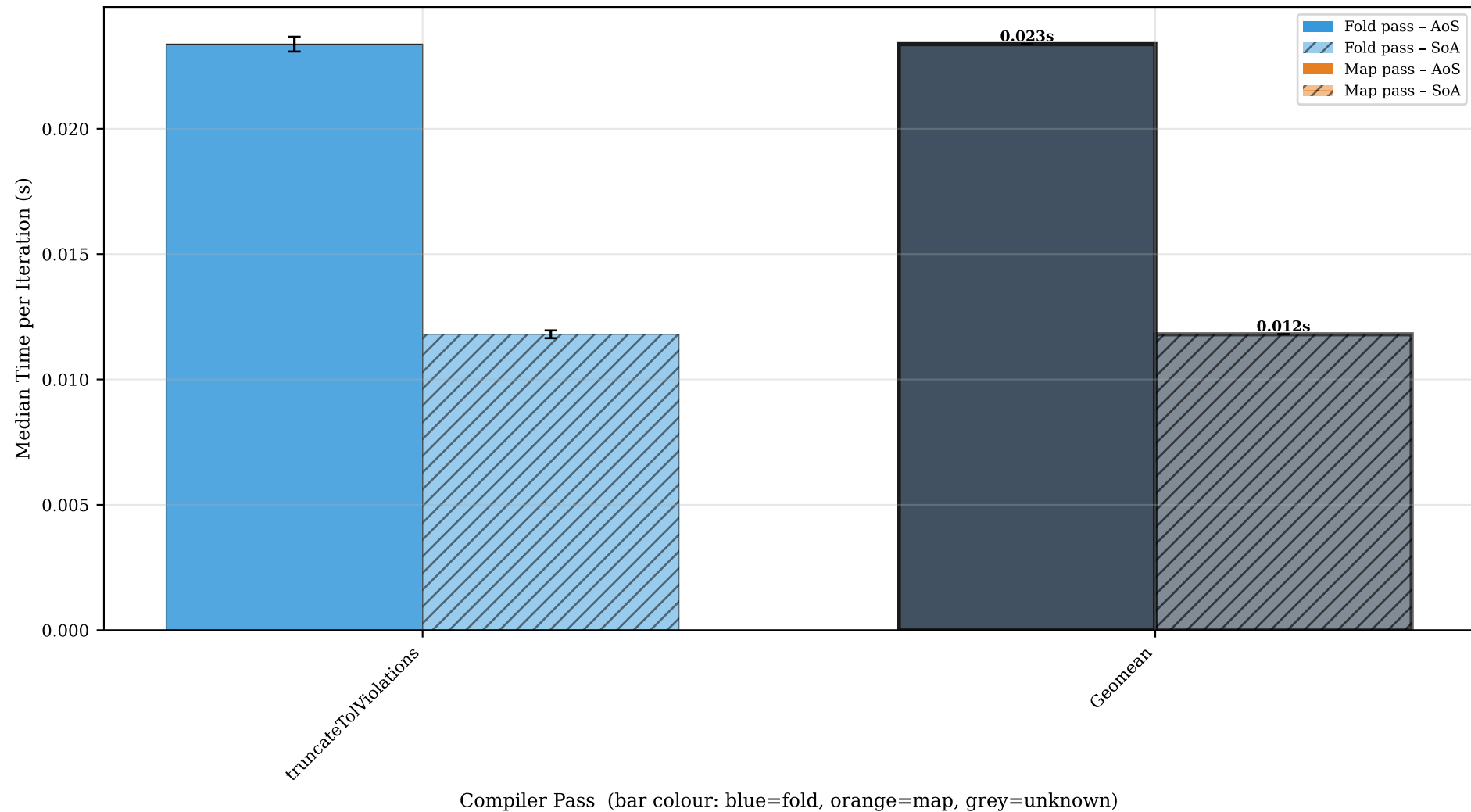
PiecewiseFunctions_truncateToViolations — AoS (solid) vs SoA (hatched), all passes (error bars = std dev, rightmost bar = geomean)
