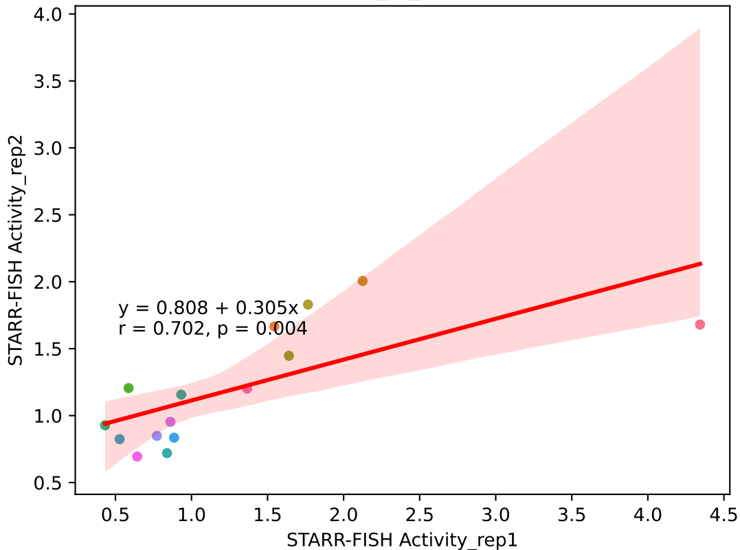
Correlation between glm_fit_result of two experiments
