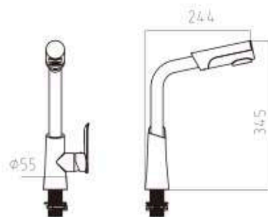
厨房感应龙头 GBL-6196D 参考价 ¥912
