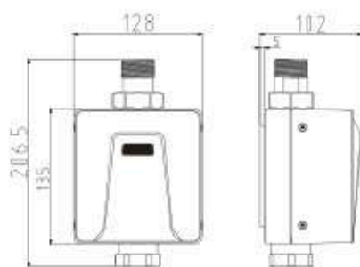
感应蹲便冲水器 GBL-6306D ¥1232 GBL-6306DM ¥1430
