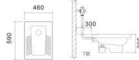
蹲便器 G13101T ¥570 G13101F ¥540
