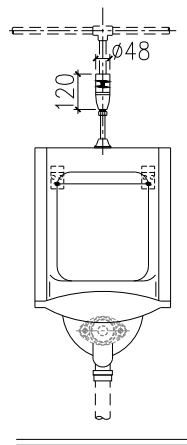
GBL-6202D Installation drawing
