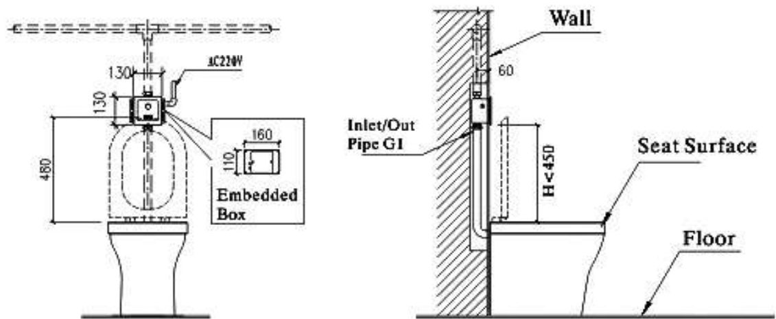
GBL-8300M Installation drawing
