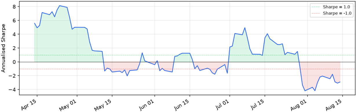
Rolling Sharpe Ratio (20-day window)
