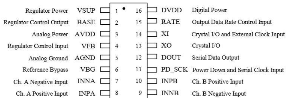
SOP-16L Package
