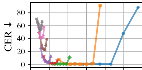
Tacotron2
