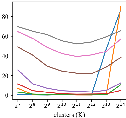
CER
