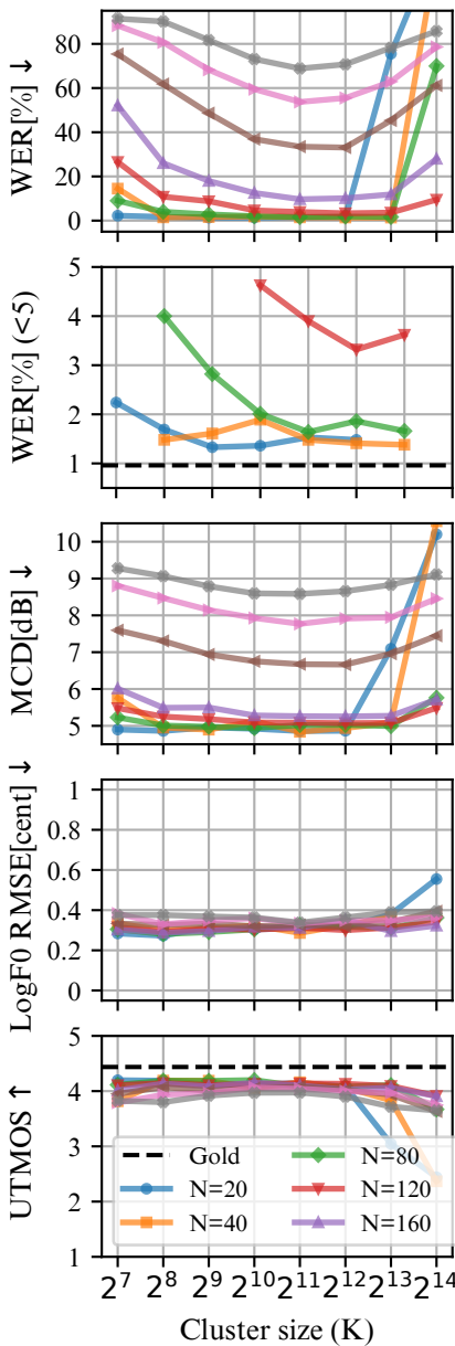
tacotron2
