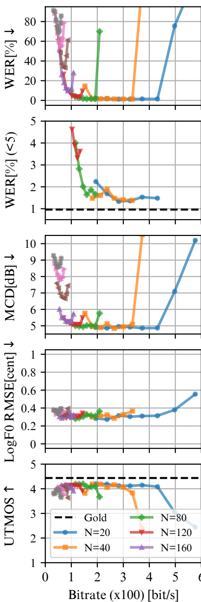
tacotron2
