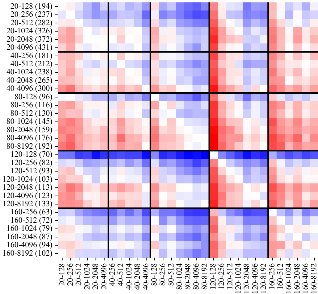
Tacotron2
