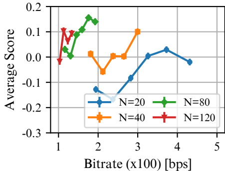
tacotron2
