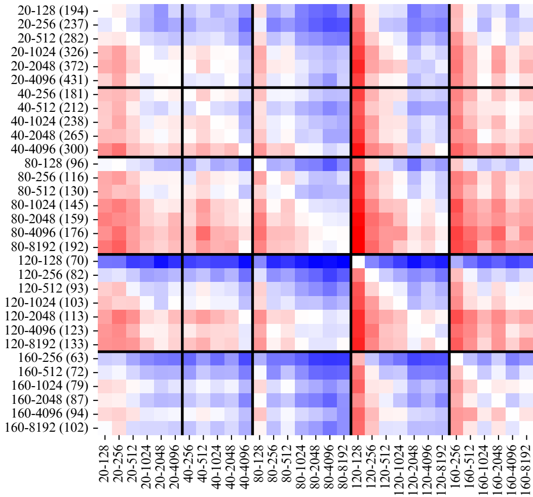
Tacotron2
