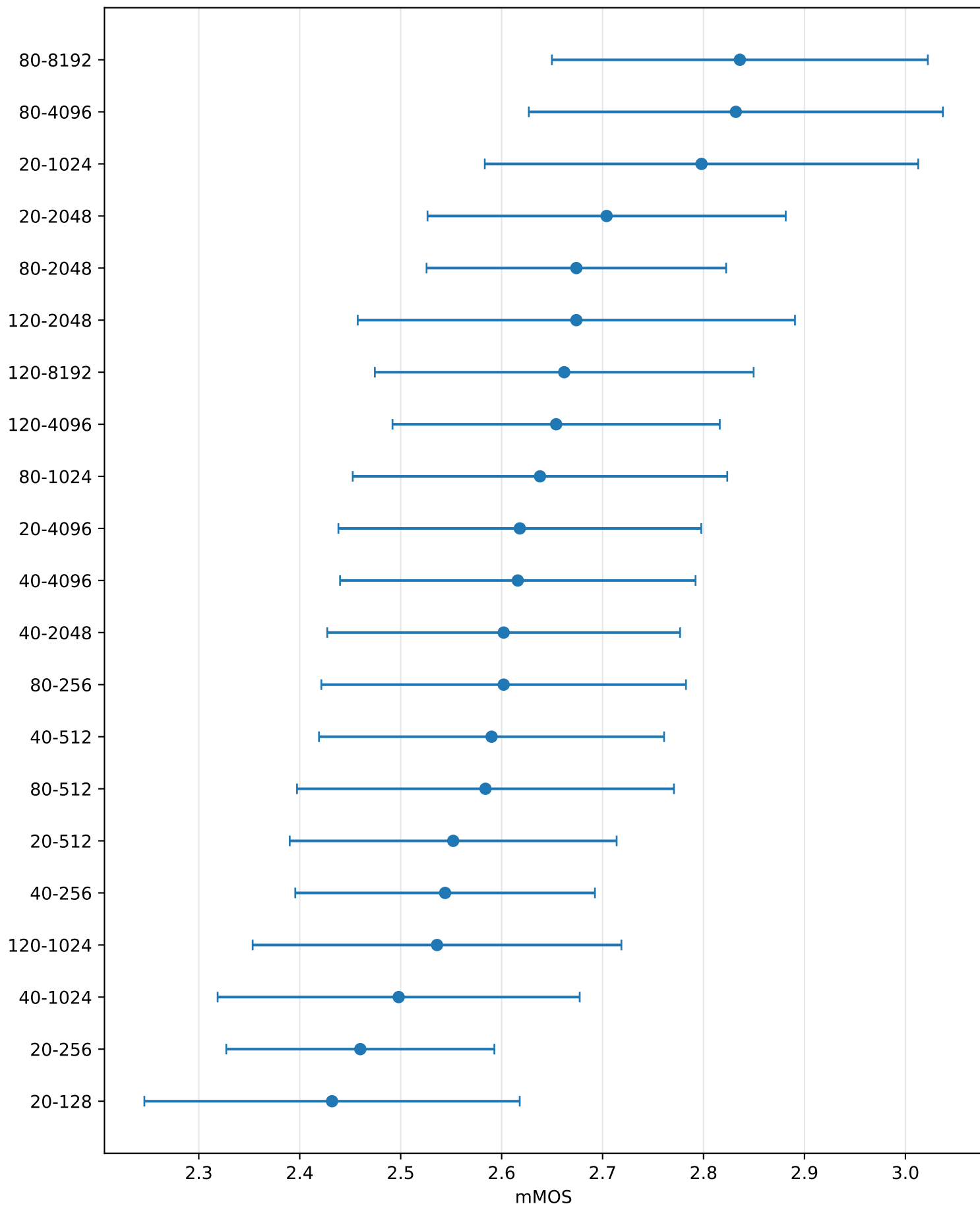
mMOS with 95% CI (sorted)
