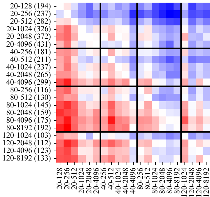
tacotron2
