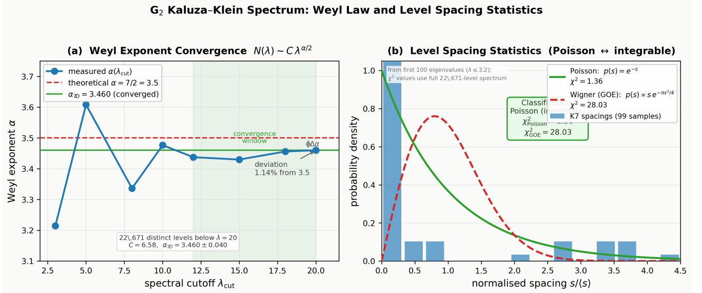
Figure 1: Weyl exponent and level spacing for the unified KK tower. (a) Convergence of the Weyl exponent \alpha(\lambda_{\text{cut}}) as the cutoff is raised: stabilisation at \alpha_{7D} = 3.460 (vs. the theoretical 7/2 = 3.5 , deviation 1.1%); the convergence window is shaded. (b) Histogram of the unfolded level spacing for the first 100 KK eigenvalues, compared to Poisson (integrable, \chi^2 = 1.36 ) and the GOE Wigner surmise ( \chi^2 = 28.0 ); the data favour Poisson by more than an order of magnitude, consistent with the adiabatic product structure.
