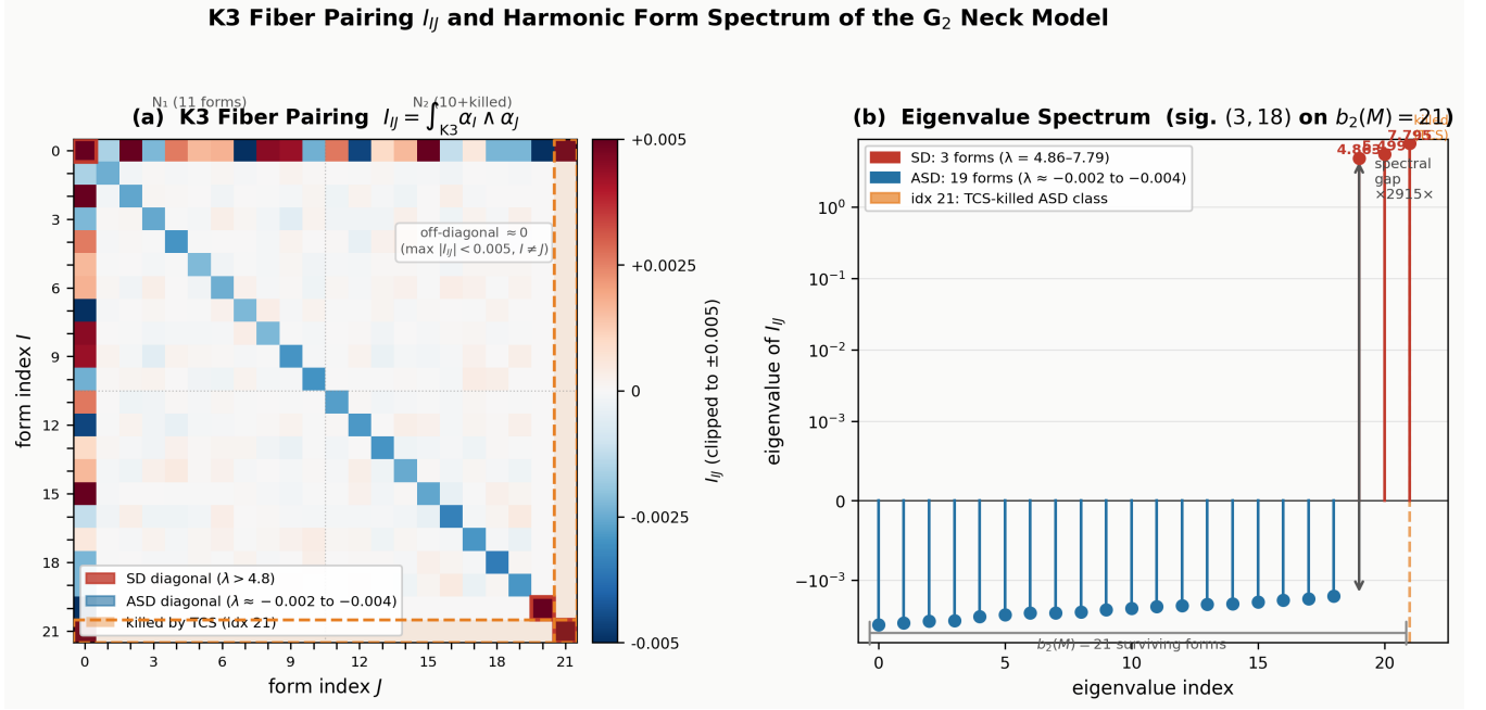
Figure 2: K3 fiber pairing I_{IJ} on the b_2(M) = 21 subspace. (a) The 22 \times 22 ambient K3 lattice pairing as a heatmap (diverging colormap, signature (3, 19)); the orange-bordered class is the lattice direction killed by TCS boundary matching, so it does not extend to a global harmonic 2-form on M . (b) Eigenvalue spectrum (signed bars) of I_{IJ} restricted to the 21 surviving global harmonic 2-forms: 3 self-dual (red, \sim 5 –8) and 18 anti-self-dual (blue, \sim -10^{-3} ), giving signature (3, 18) and the SD/ASD spectral gap of \sim 2,210 .
