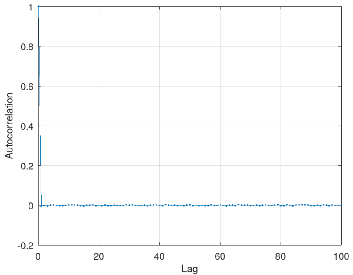
Autocorrelation of Key Stream (LSS)
