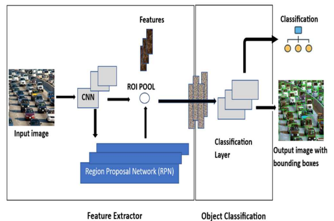
Fig. 3. Architecture of FR-CNN model for vehicle detection
