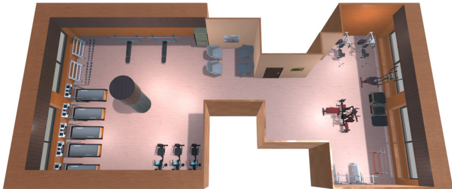
Gym 01
